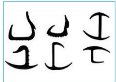
J-TYPE BEADINGS
